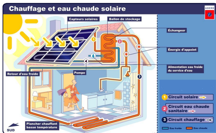
Figure 13: Chauffe-eau solaire
